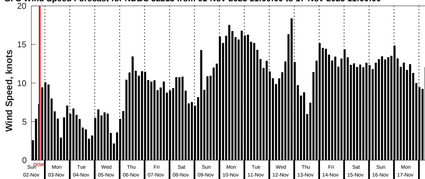
GFS Wind Speed Forecast for NDBC 52213 from 01-Nov-2025 11:00:00 to 17-Nov-2025 11:00:00
