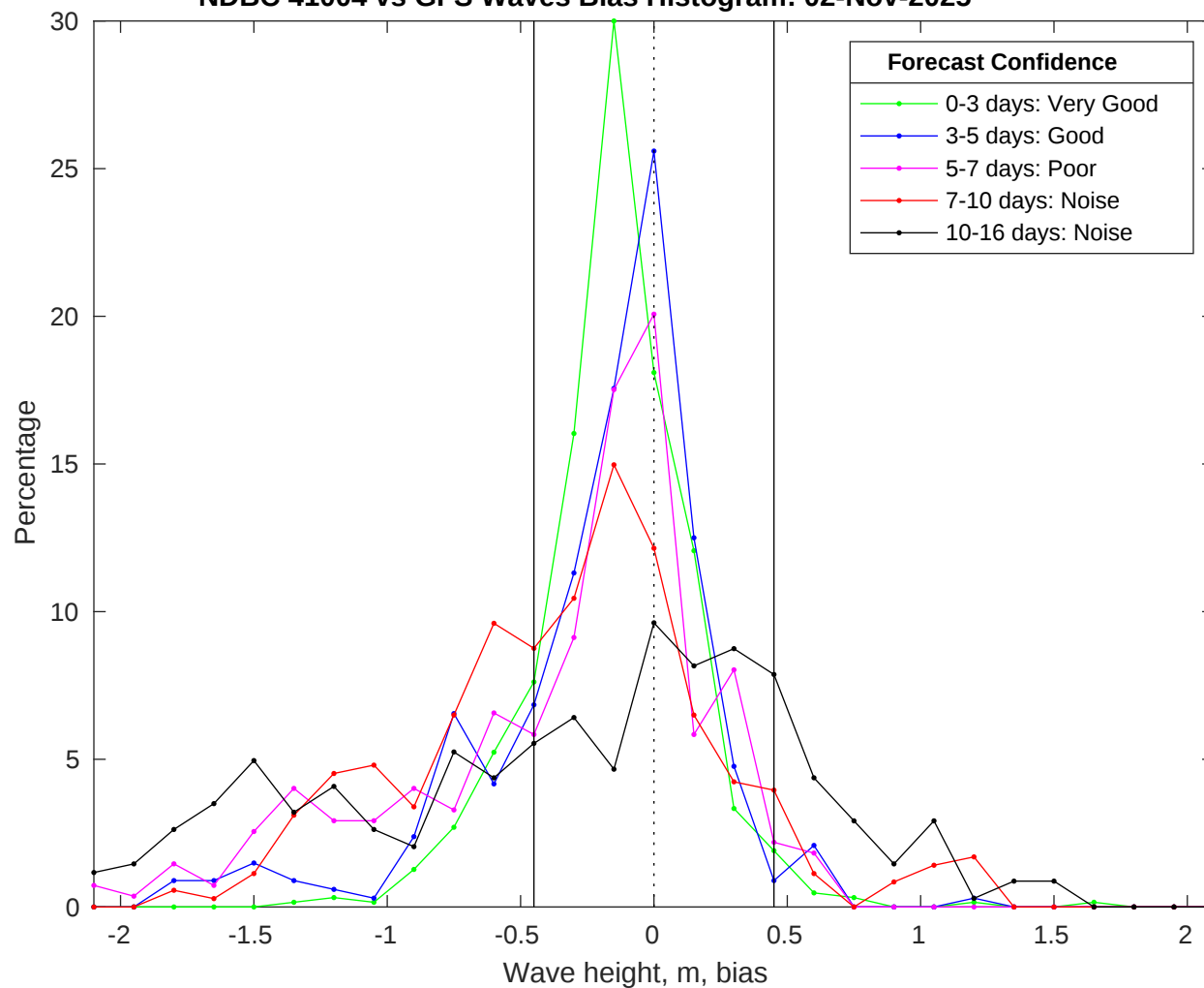
NDBC 41004 vs GFS Waves Bias Histogram: 02-Nov-2025
