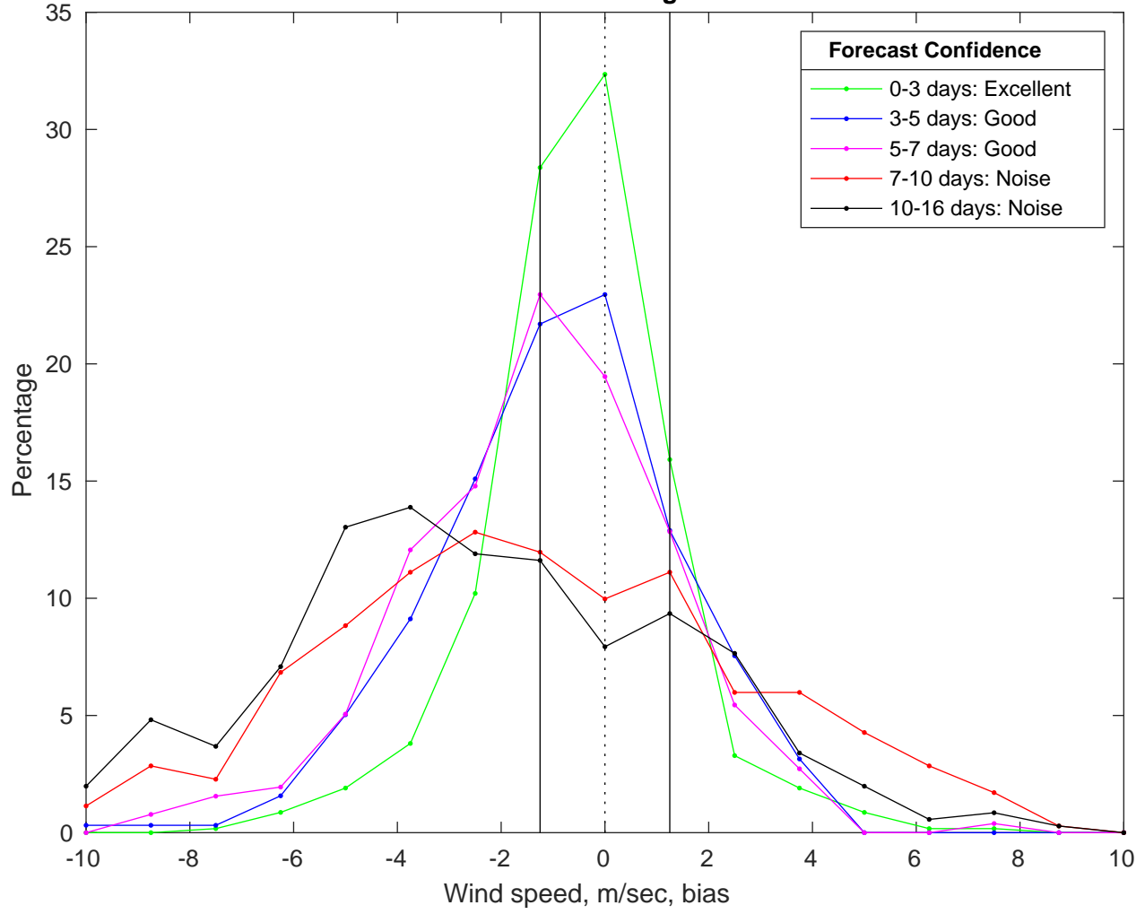
NDBC 41004 vs GFS Winds Bias Histogram: 02-Nov-2025
