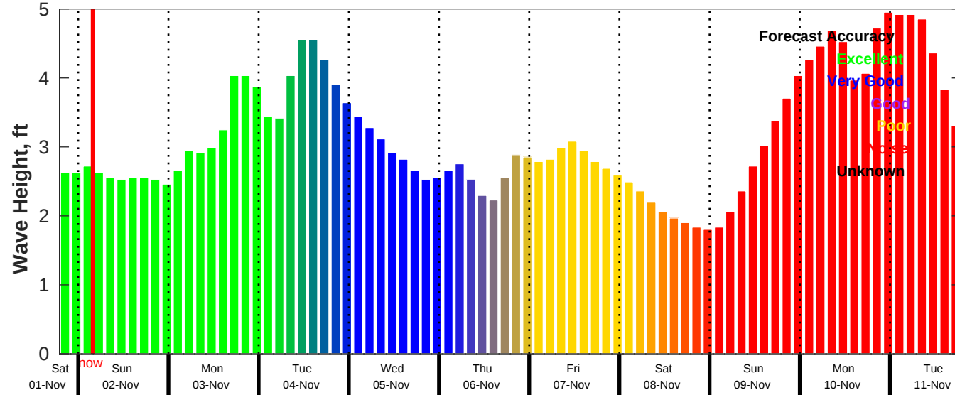
CMEMS Wave Forecast for NDBC 41004 from 01-Nov-2025 19:00:00 to 11-Nov-2025 19:00:00
