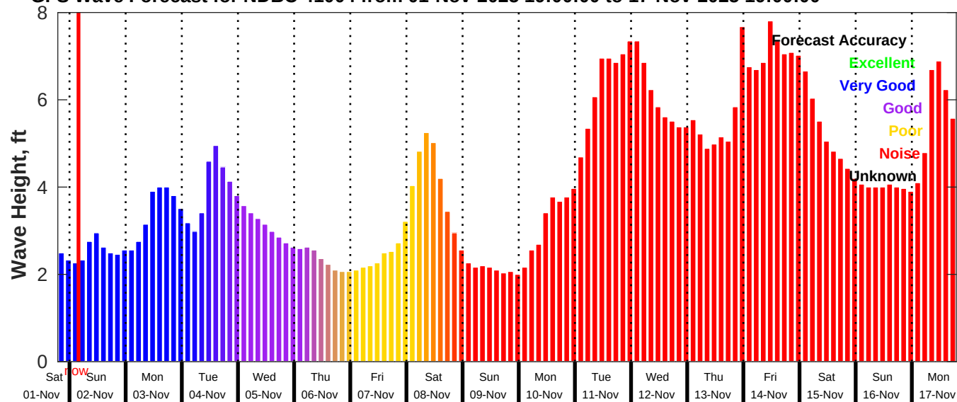
GFS Wave Forecast for NDBC 41004 from 01-Nov-2025 19:00:00 to 17-Nov-2025 19:00:00
