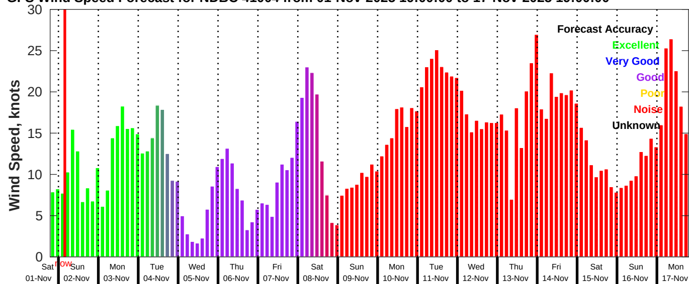
GFS Wind Speed Forecast for NDBC 41004 from 01-Nov-2025 19:00:00 to 17-Nov-2025 19:00:00
