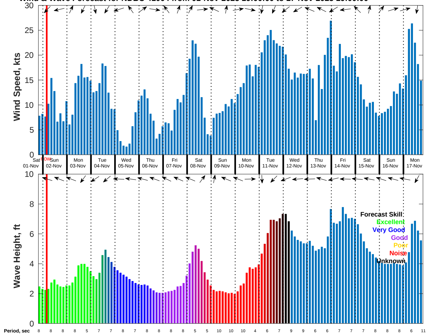
Wind & Wave Forecast for NDBC 41004 from 01-Nov-2025 19:00:00 to 17-Nov-2025 19:00:00
