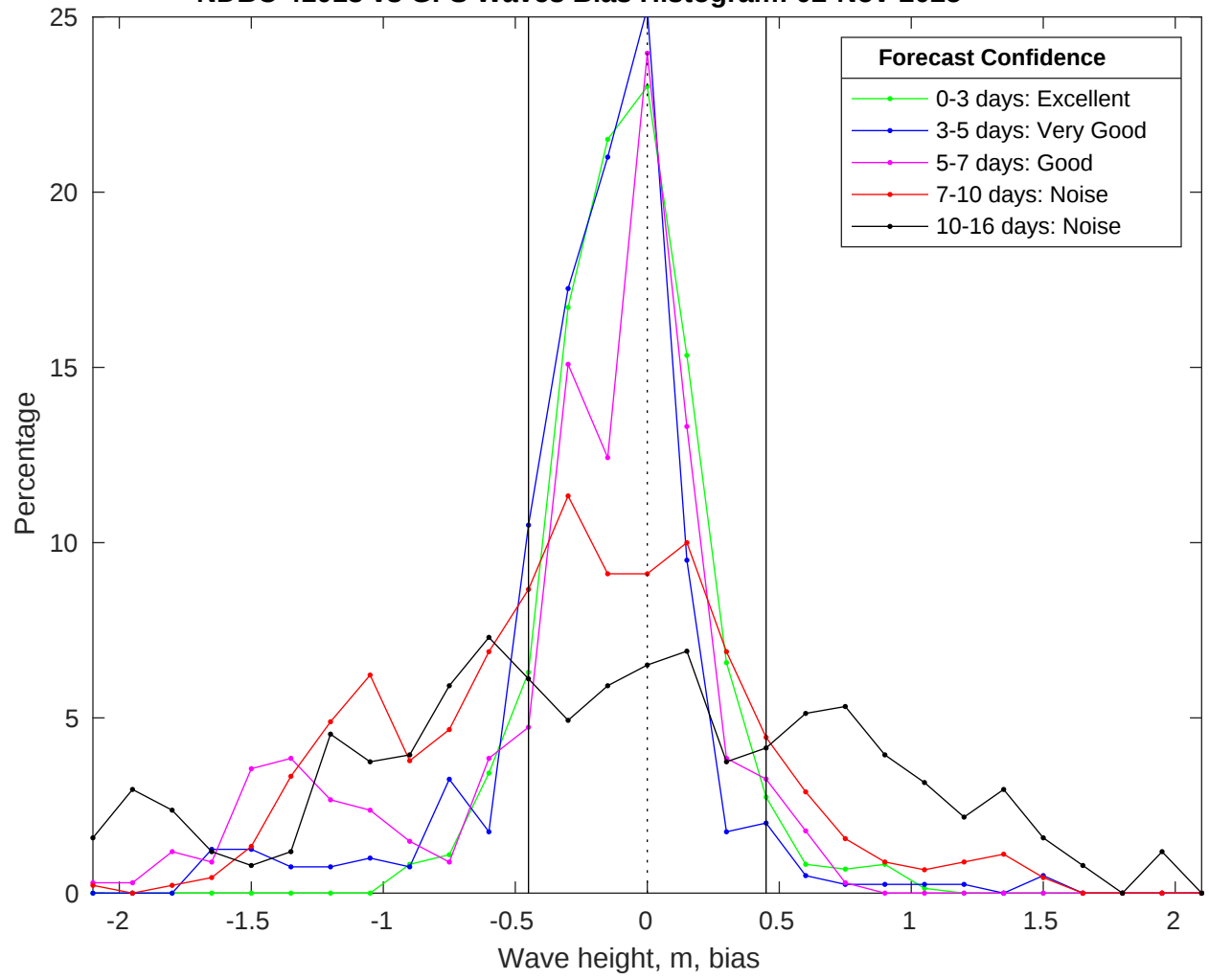
NDBC 41013 vs GFS Waves Bias Histogram: 02-Nov-2025
