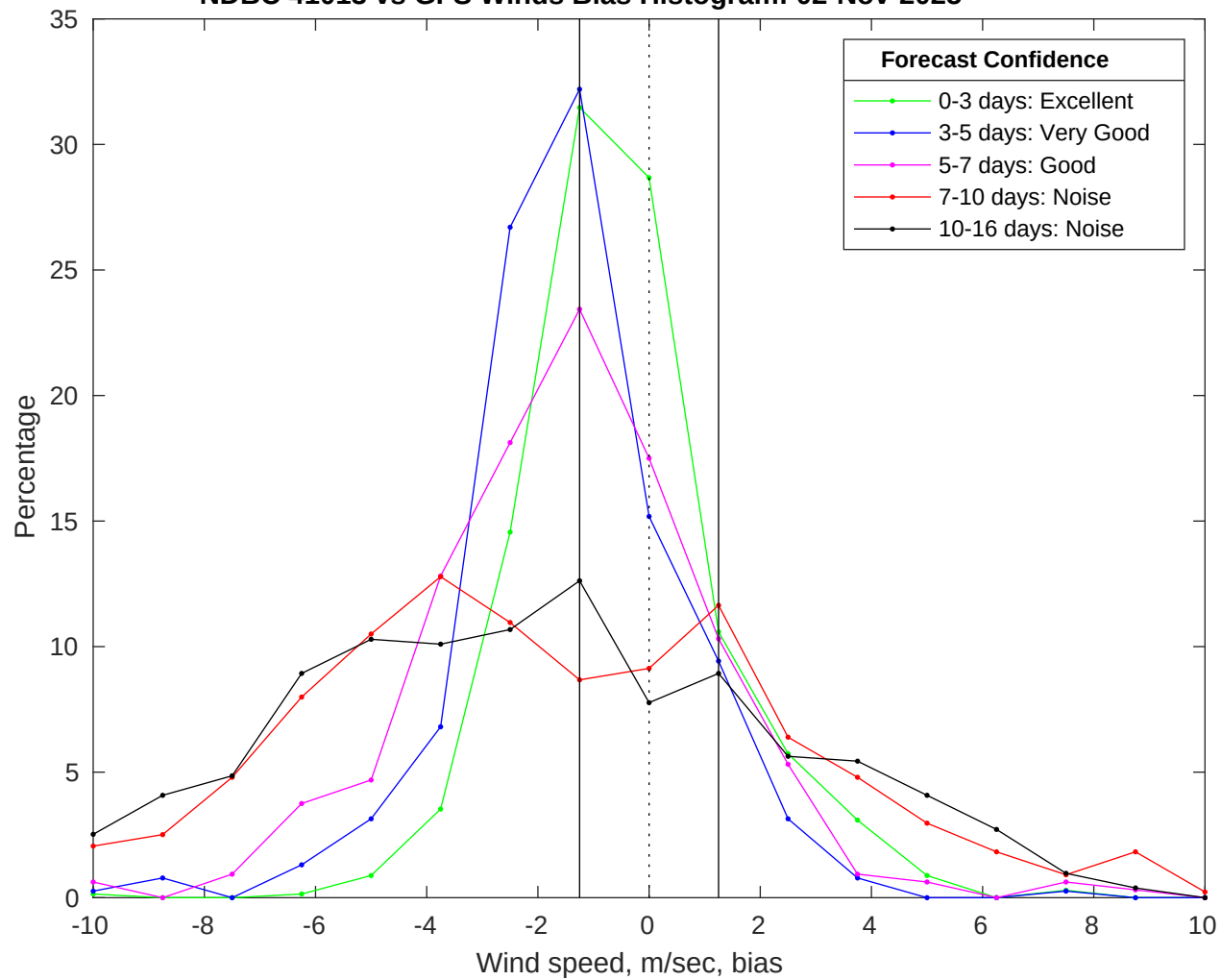
NDBC 41013 vs GFS Winds Bias Histogram: 02-Nov-2025
