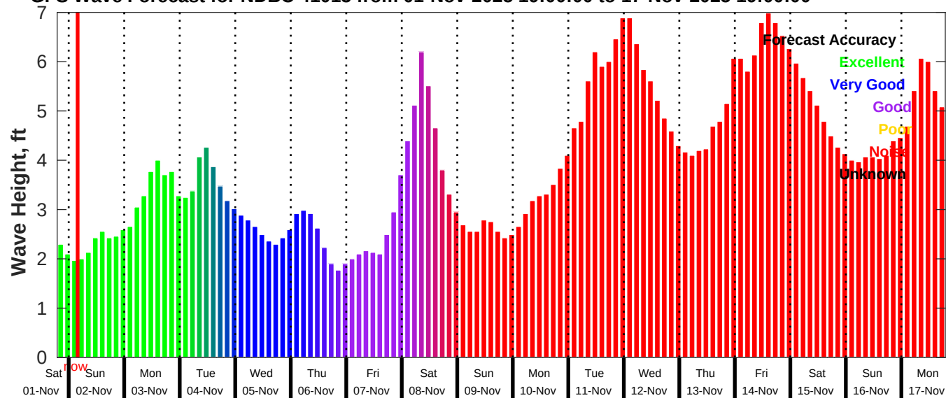
GFS Wave Forecast for NDBC 41013 from 01-Nov-2025 19:00:00 to 17-Nov-2025 19:00:00
