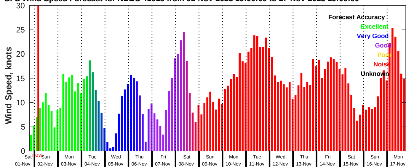
GFS Wind Speed Forecast for NDBC 41013 from 01-Nov-2025 19:00:00 to 17-Nov-2025 19:00:00
