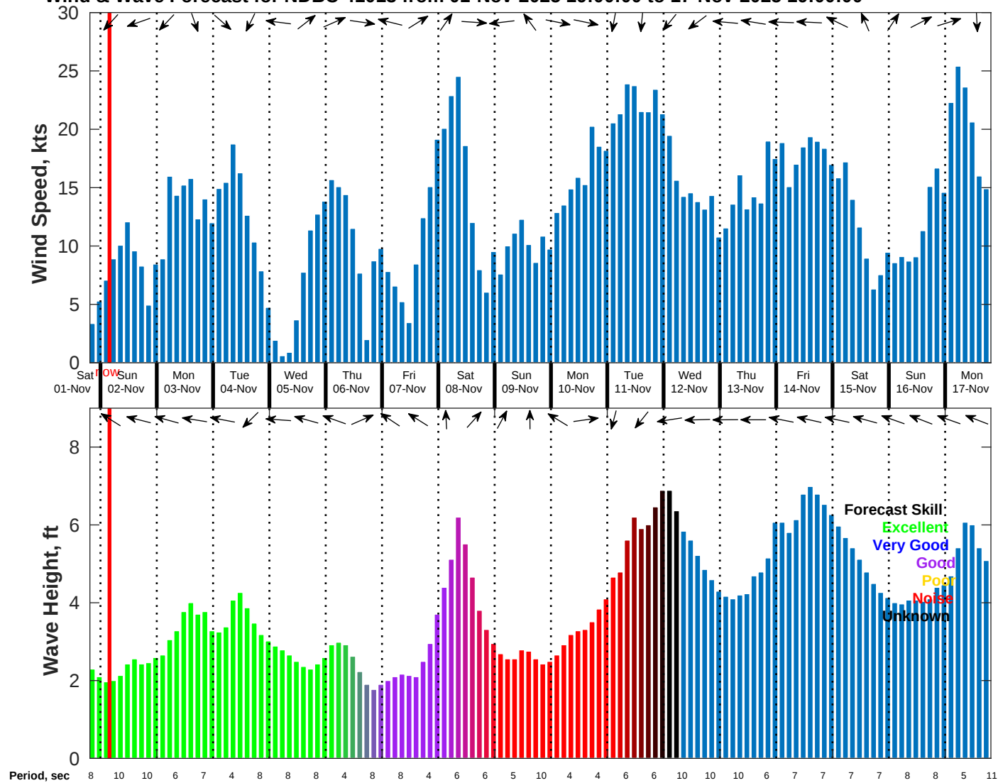
Wind & Wave Forecast for NDBC 41013 from 01-Nov-2025 19:00:00 to 17-Nov-2025 19:00:00
