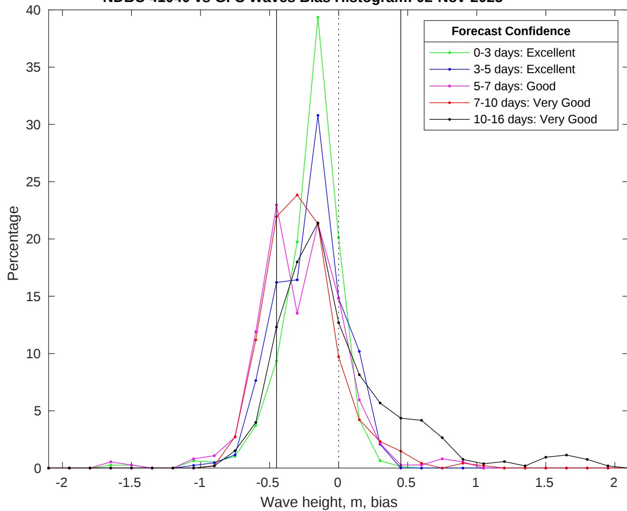
NDBC 41040 vs GFS Waves Bias Histogram: 02-Nov-2025
