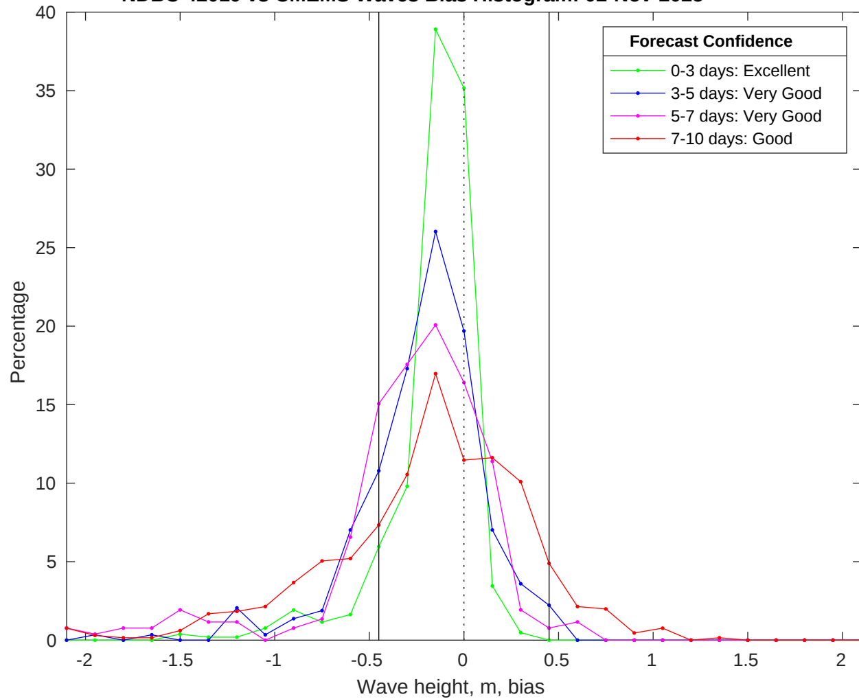
NDBC 42019 vs CMEMS Waves Bias Histogram: 02-Nov-2025
