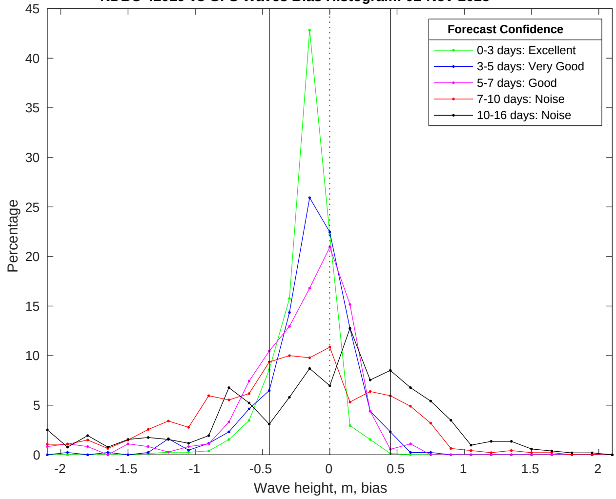
NDBC 42019 vs GFS Waves Bias Histogram: 02-Nov-2025
