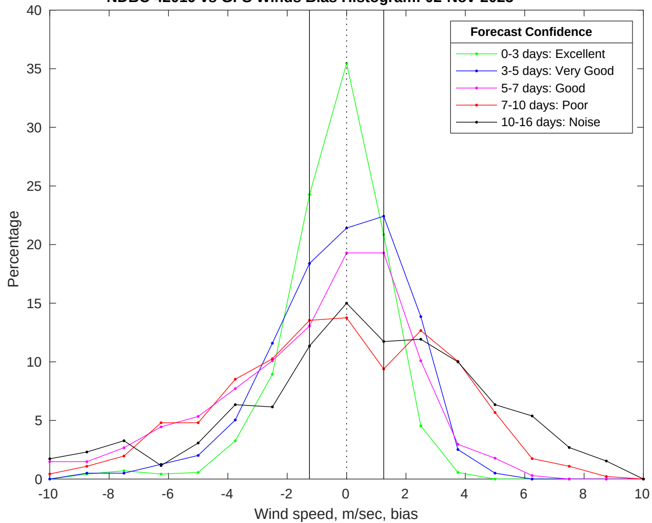
NDBC 42019 vs GFS Winds Bias Histogram: 02-Nov-2025
