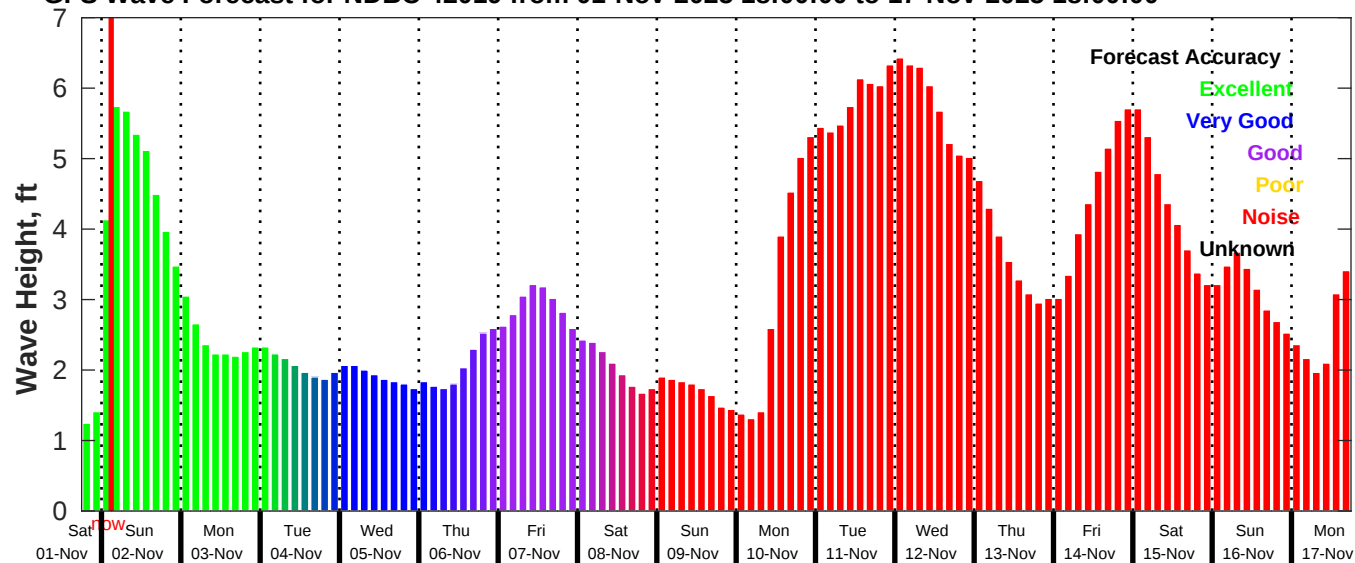
GFS Wave Forecast for NDBC 42019 from 01-Nov-2025 18:00:00 to 17-Nov-2025 18:00:00
