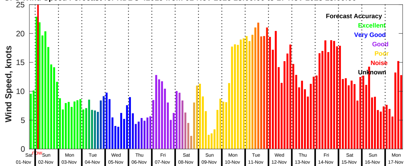
GFS Wind Speed Forecast for NDBC 42019 from 01-Nov-2025 18:00:00 to 17-Nov-2025 18:00:00
