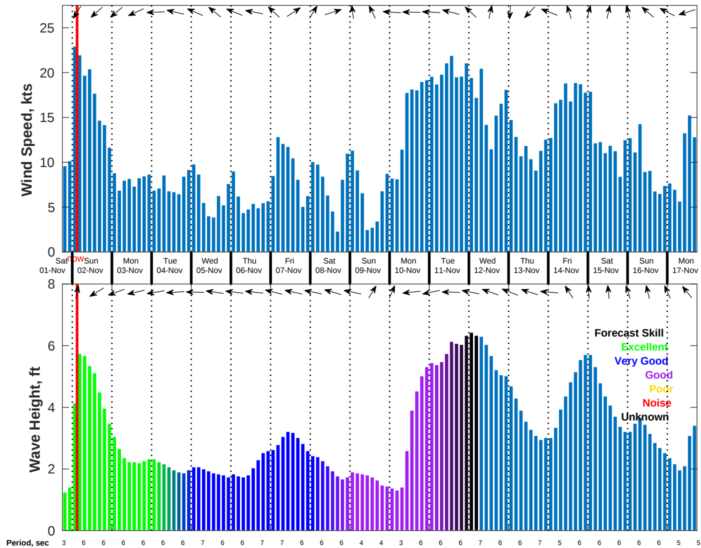
Wind & Wave Forecast for NDBC 42019 from 01-Nov-2025 18:00:00 to 17-Nov-2025 18:00:00
