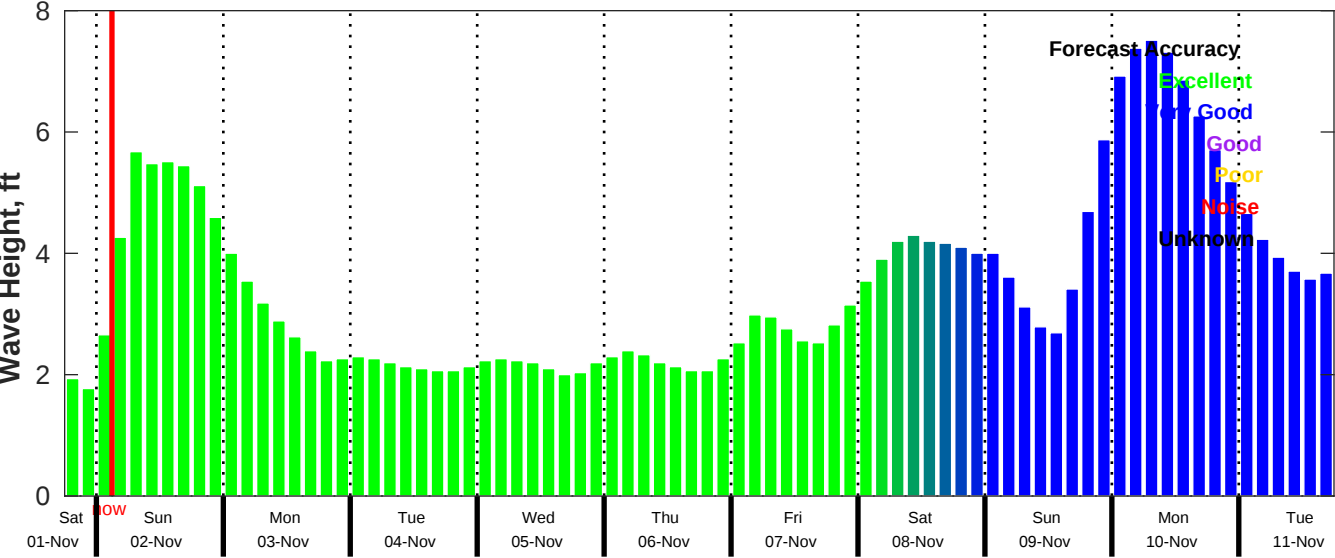
CMEMS Wave Forecast for NDBC 42020 from 01-Nov-2025 18:00:00 to 11-Nov-2025 18:00:00
