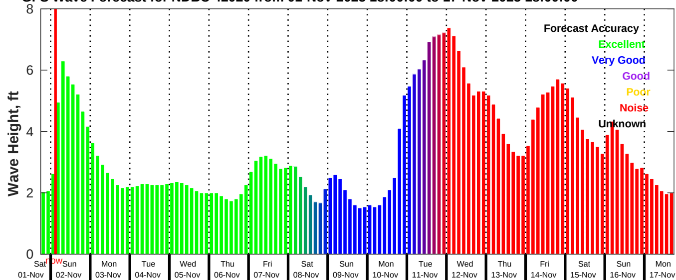
GFS Wave Forecast for NDBC 42020 from 01-Nov-2025 18:00:00 to 17-Nov-2025 18:00:00
