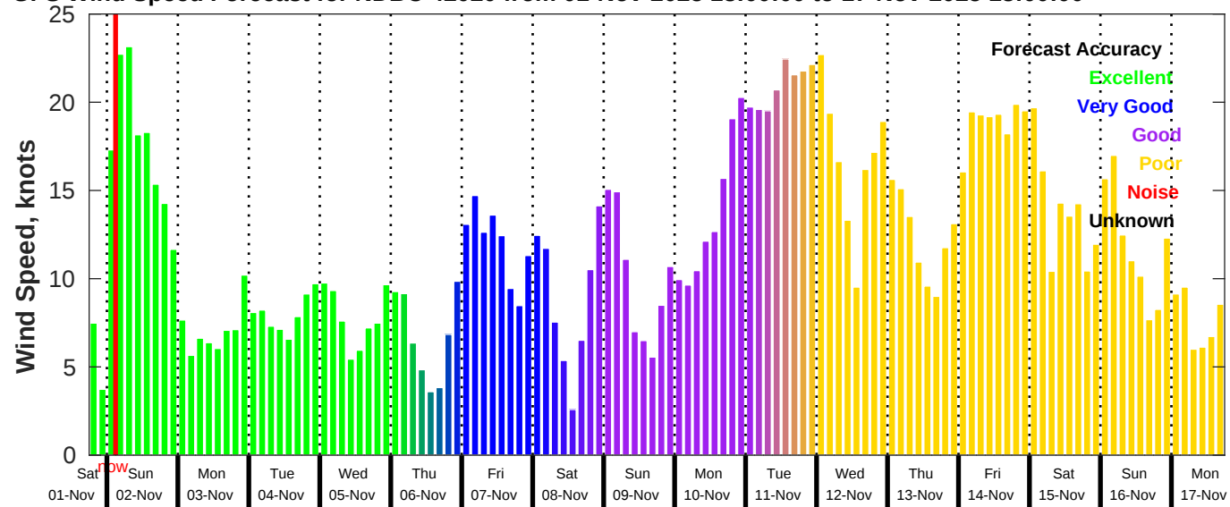
GFS Wind Speed Forecast for NDBC 42020 from 01-Nov-2025 18:00:00 to 17-Nov-2025 18:00:00
