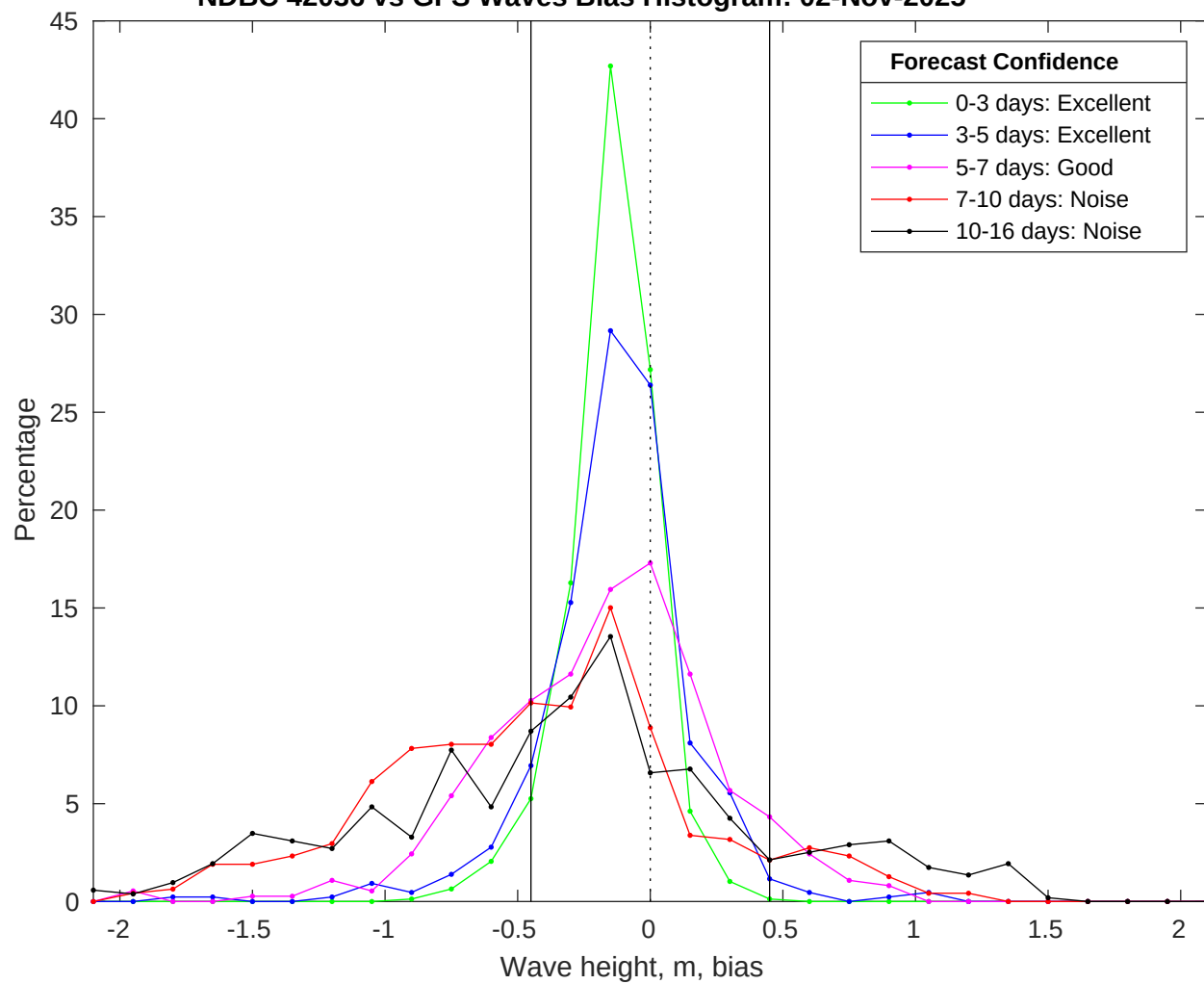
NDBC 42036 vs GFS Waves Bias Histogram: 02-Nov-2025
