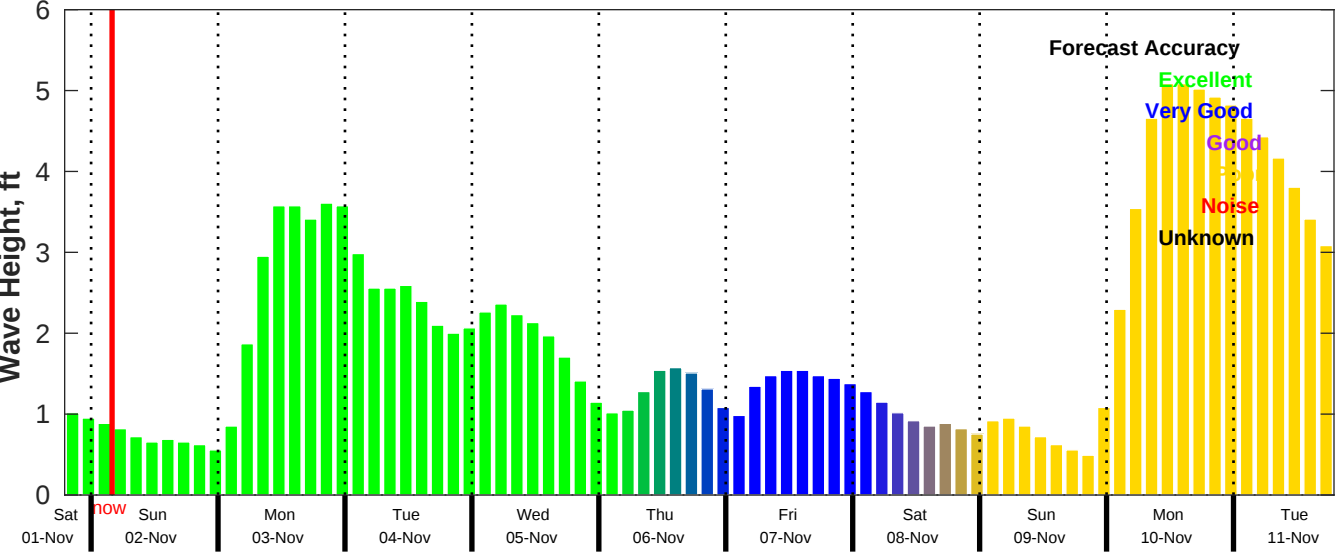
CMEMS Wave Forecast for NDBC 42036 from 01-Nov-2025 19:00:00 to 11-Nov-2025 19:00:00
