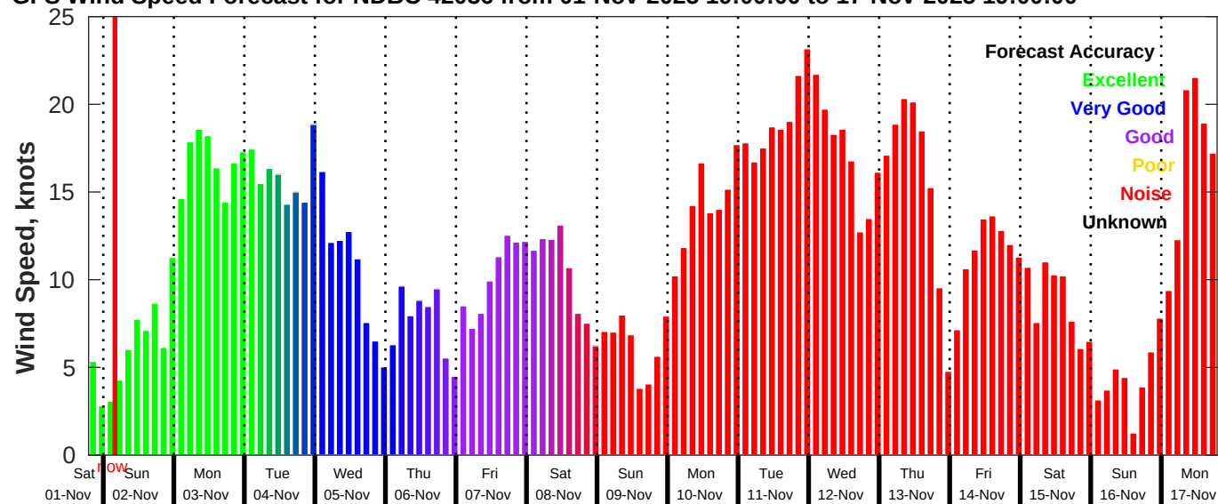
GFS Wind Speed Forecast for NDBC 42036 from 01-Nov-2025 19:00:00 to 17-Nov-2025 19:00:00
