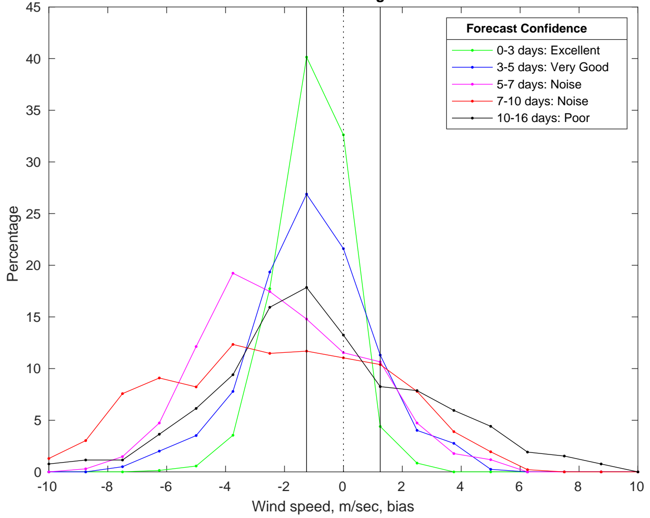
NDBC 42040 vs GFS Winds Bias Histogram: 02-Nov-2025
