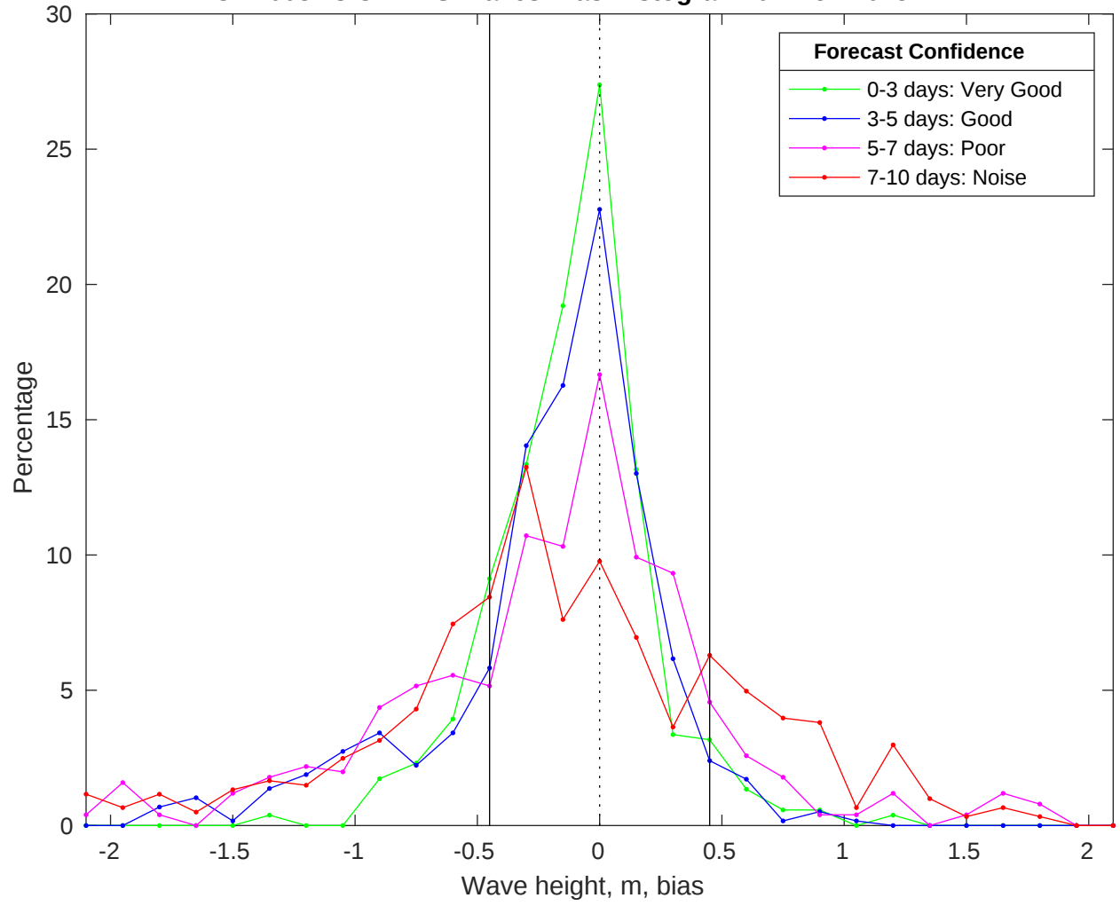
NDBC 44008 vs CMEMS Waves Bias Histogram: 02-Nov-2025
