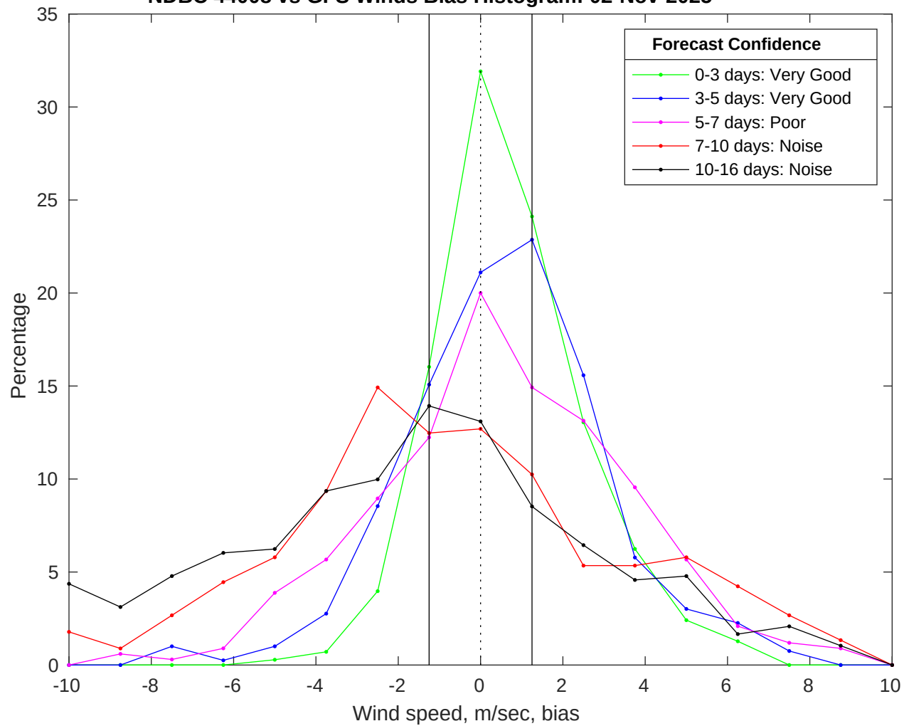
NDBC 44008 vs GFS Winds Bias Histogram: 02-Nov-2025
