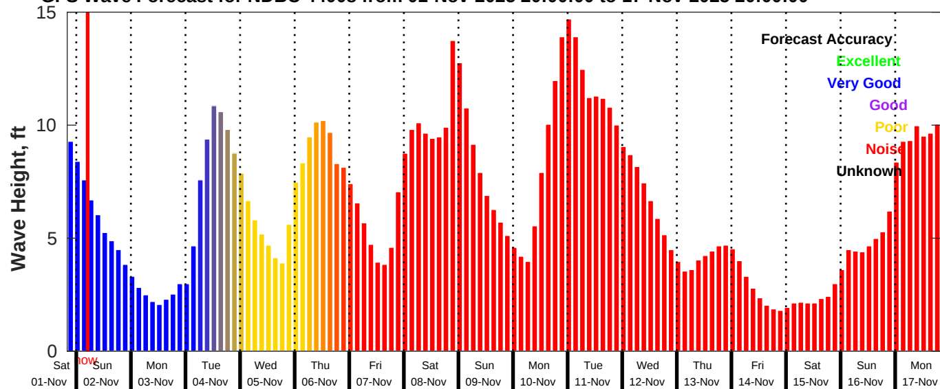
GFS Wave Forecast for NDBC 44008 from 01-Nov-2025 20:00:00 to 17-Nov-2025 20:00:00
