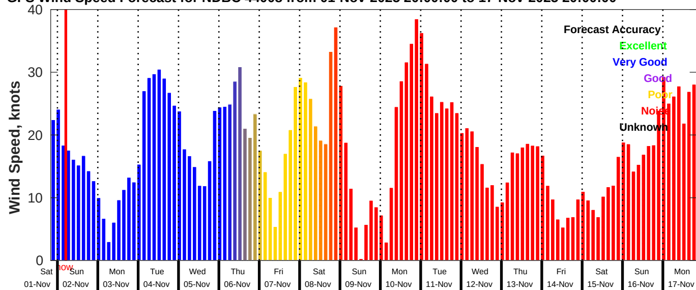
GFS Wind Speed Forecast for NDBC 44008 from 01-Nov-2025 20:00:00 to 17-Nov-2025 20:00:00
