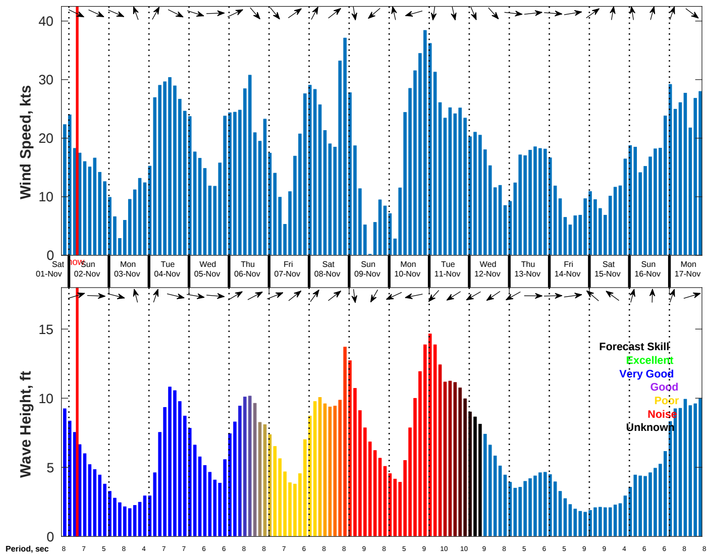
Wind & Wave Forecast for NDBC 44008 from 01-Nov-2025 20:00:00 to 17-Nov-2025 20:00:00
