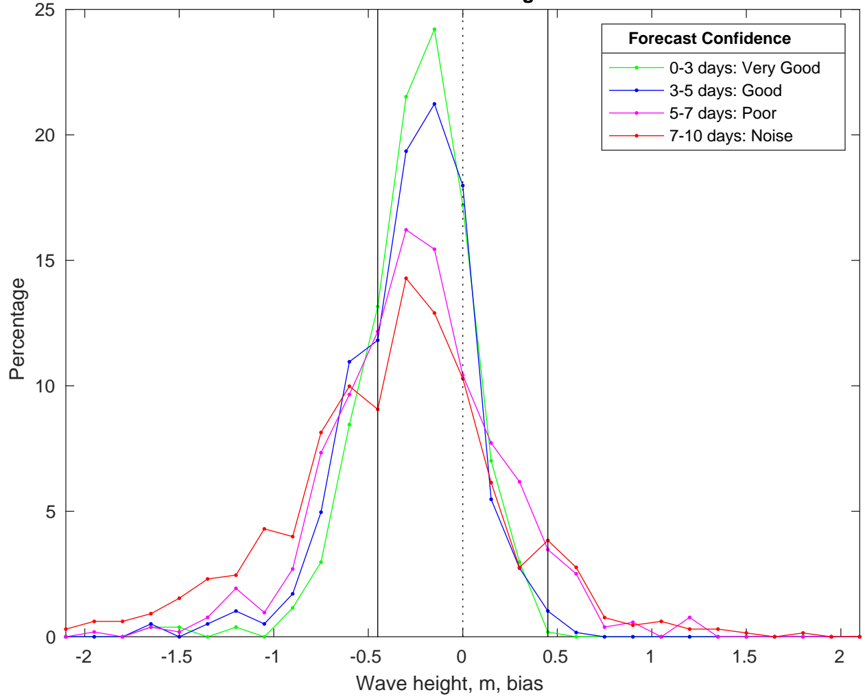
NDBC 46011 vs CMEMS Waves Bias Histogram: 02-Nov-2025
