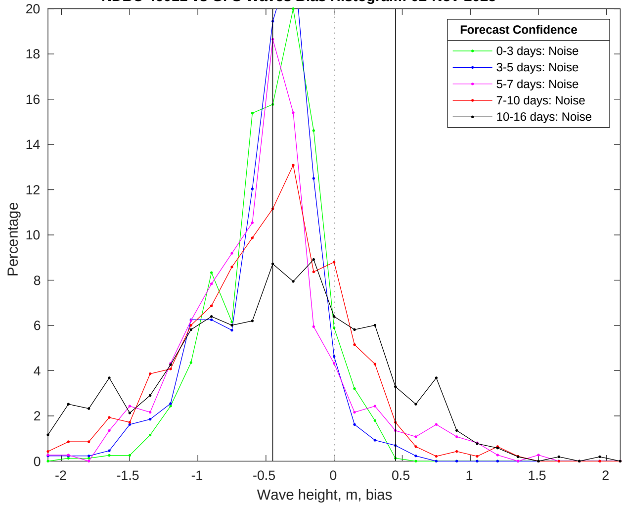
NDBC 46011 vs GFS Waves Bias Histogram: 02-Nov-2025
