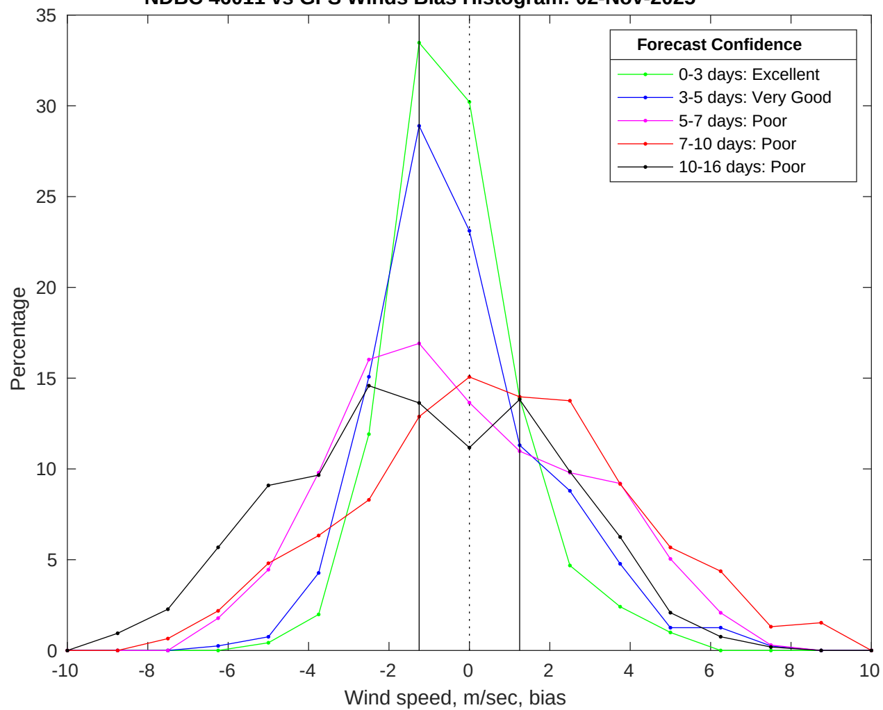
NDBC 46011 vs GFS Winds Bias Histogram: 02-Nov-2025
