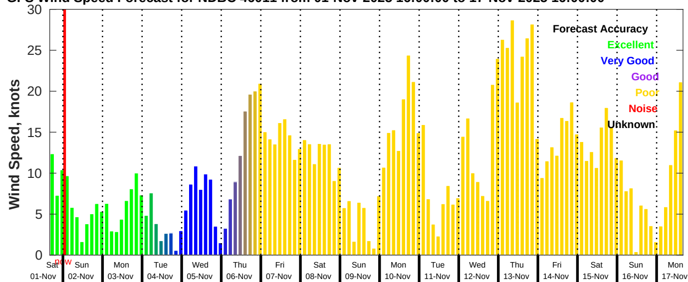
GFS Wind Speed Forecast for NDBC 46011 from 01-Nov-2025 16:00:00 to 17-Nov-2025 16:00:00
