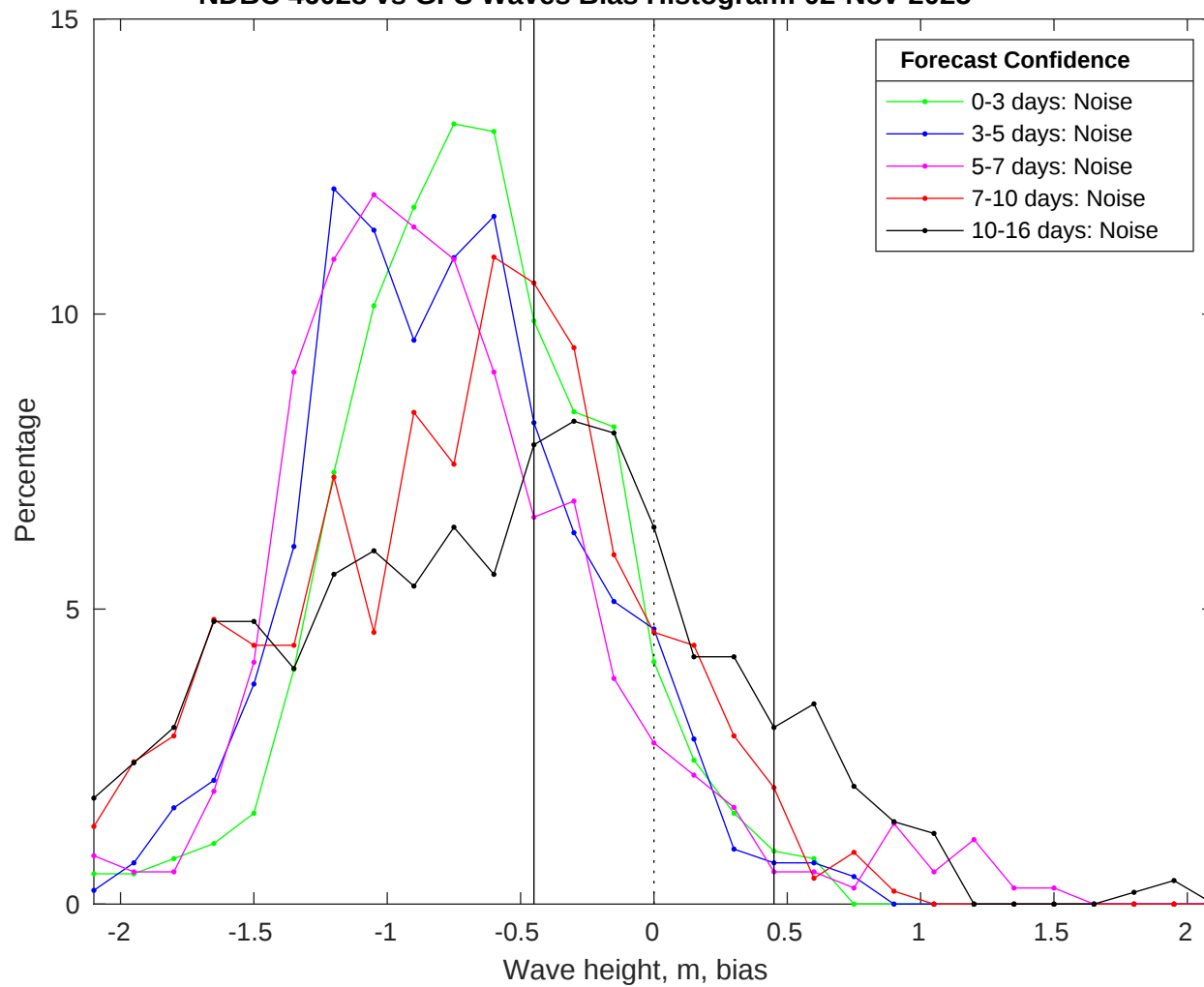
NDBC 46028 vs GFS Waves Bias Histogram: 02-Nov-2025
