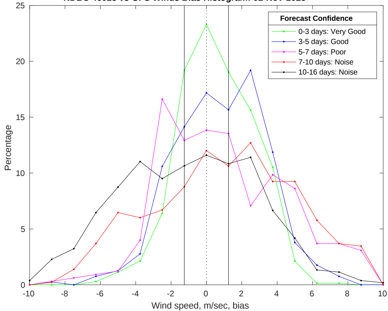
NDBC 46028 vs GFS Winds Bias Histogram: 02-Nov-2025
