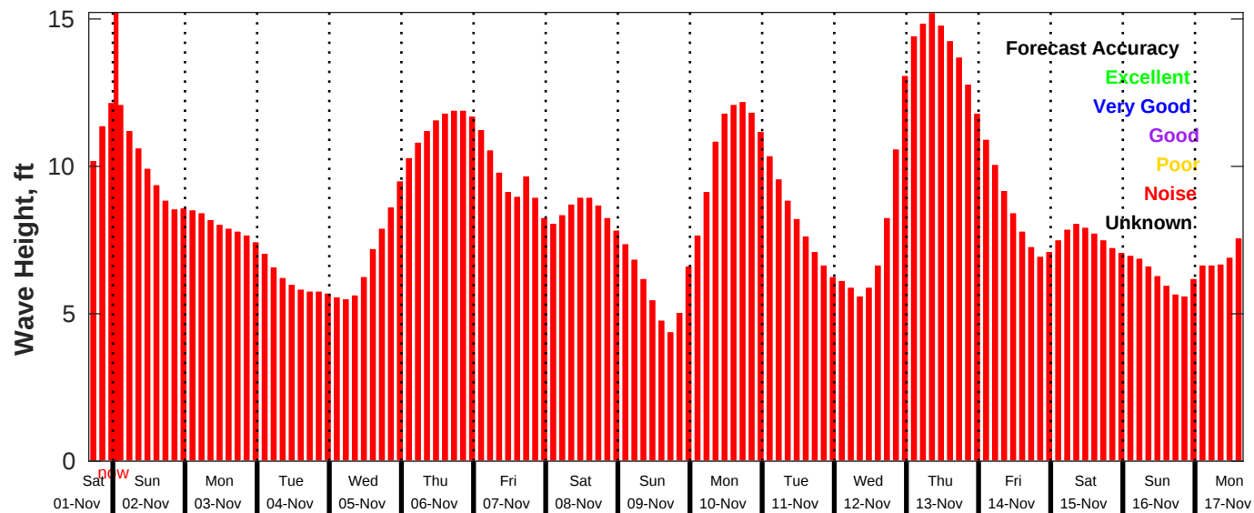
GFS Wave Forecast for NDBC 46028 from 01-Nov-2025 16:00:00 to 17-Nov-2025 16:00:00
