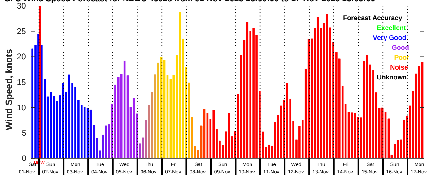
GFS Wind Speed Forecast for NDBC 46028 from 01-Nov-2025 16:00:00 to 17-Nov-2025 16:00:00
