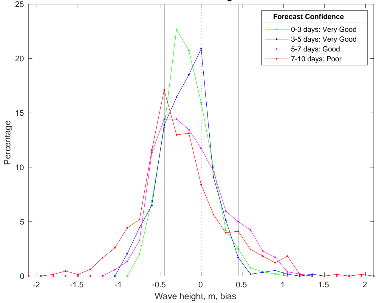
NDBC 46054 vs CMEMS Waves Bias Histogram: 02-Nov-2025
