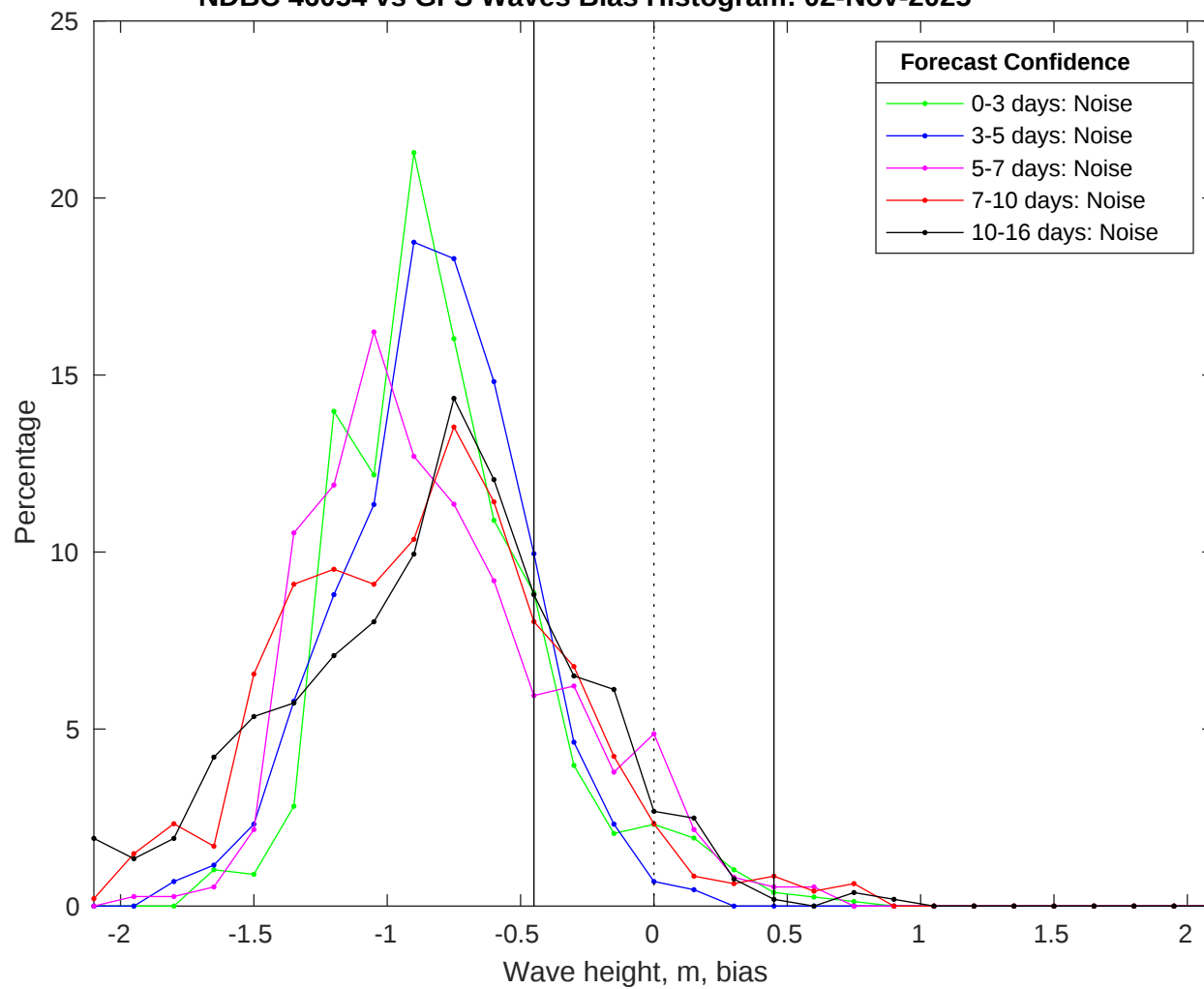
NDBC 46054 vs GFS Waves Bias Histogram: 02-Nov-2025
