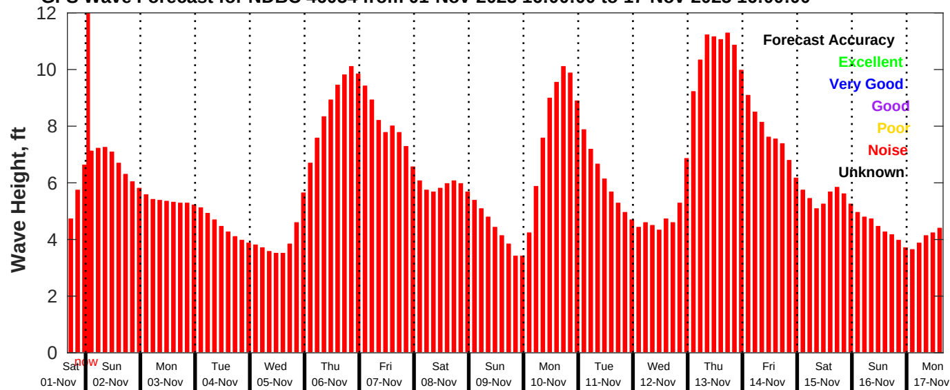
GFS Wave Forecast for NDBC 46054 from 01-Nov-2025 16:00:00 to 17-Nov-2025 16:00:00
