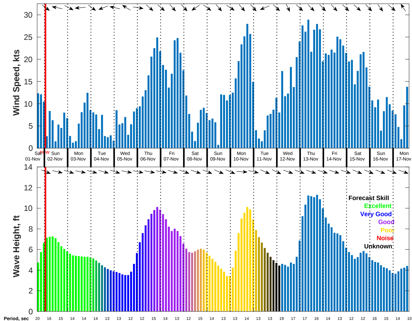
Wind & Wave Forecast for NDBC 46054 from 01-Nov-2025 16:00:00 to 17-Nov-2025 16:00:00
