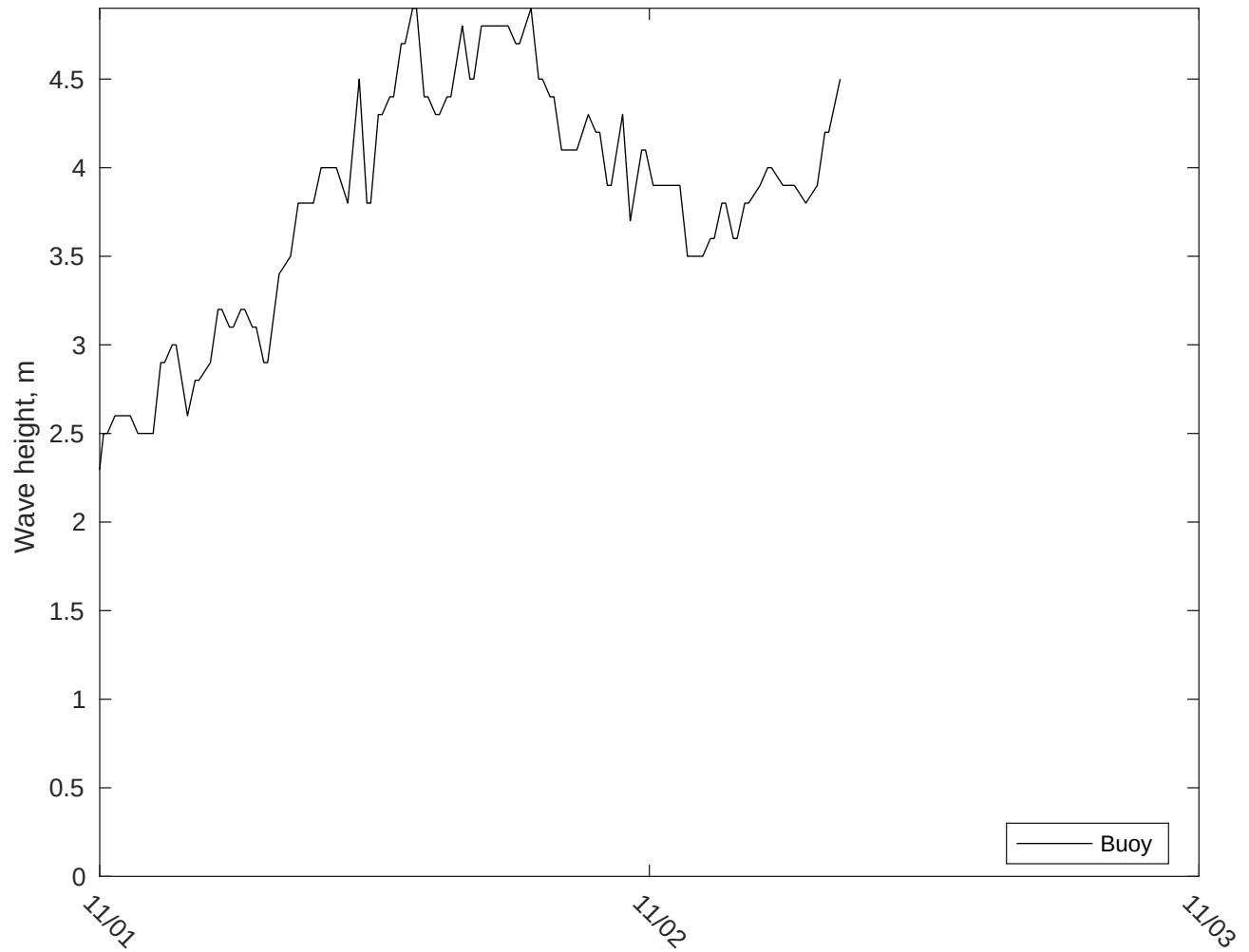
NDBC 46059 vs CMEMS Waves: 10 to 16 day forecast
