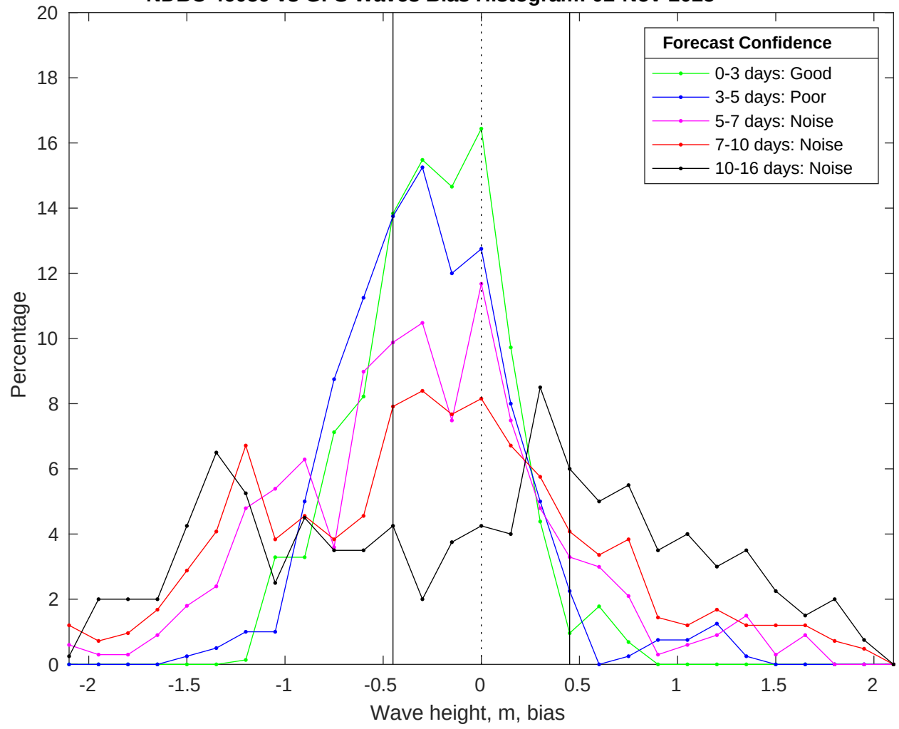
NDBC 46059 vs GFS Waves Bias Histogram: 02-Nov-2025
