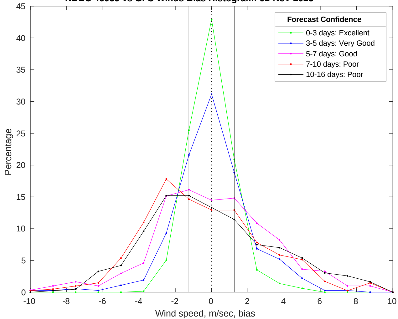
NDBC 46059 vs GFS Winds Bias Histogram: 02-Nov-2025
