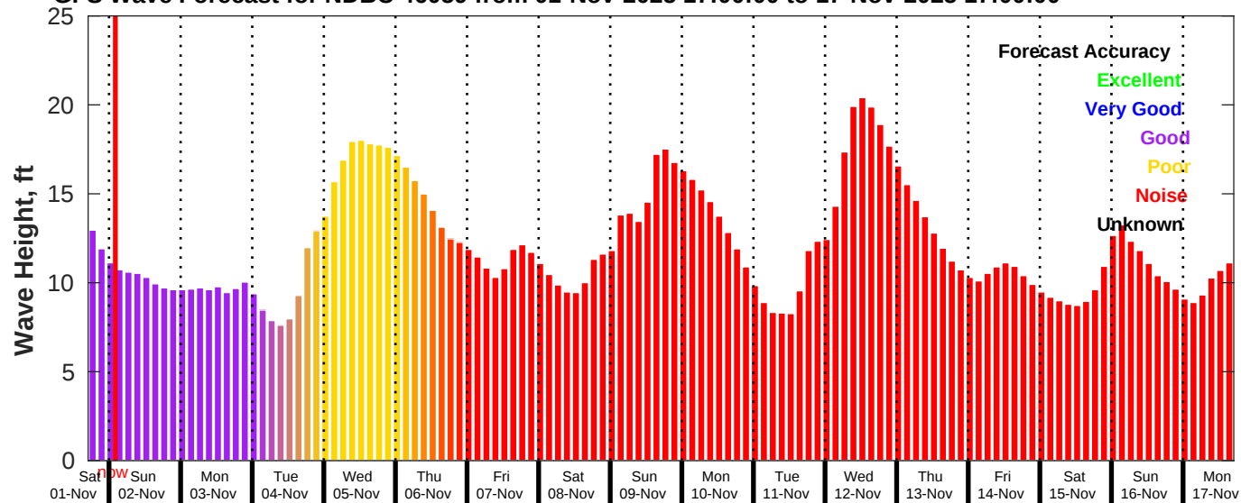
GFS Wave Forecast for NDBC 46059 from 01-Nov-2025 17:00:00 to 17-Nov-2025 17:00:00
