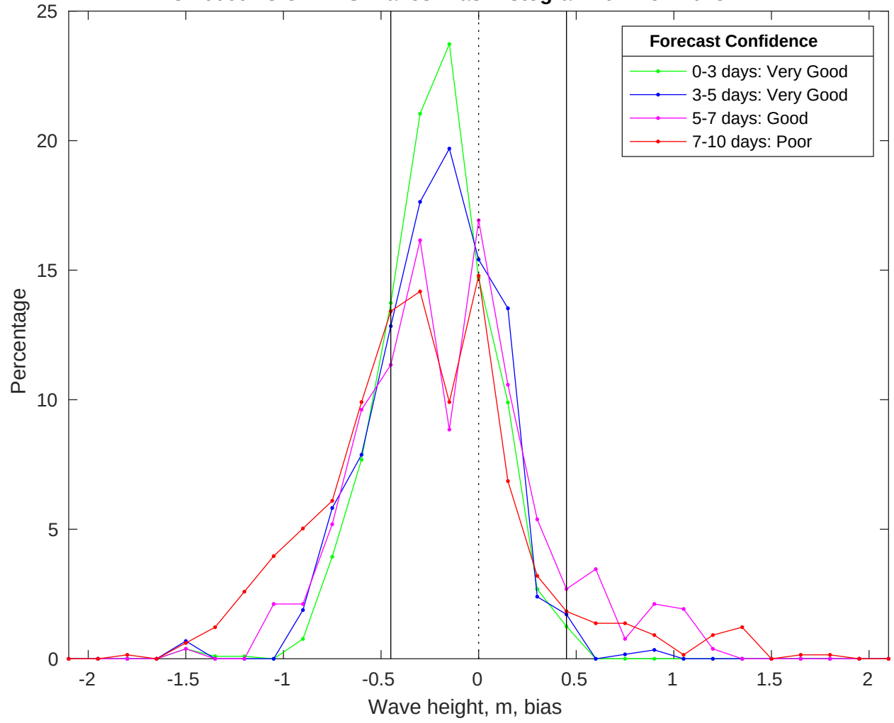
NDBC 46069 vs CMEMS Waves Bias Histogram: 02-Nov-2025
