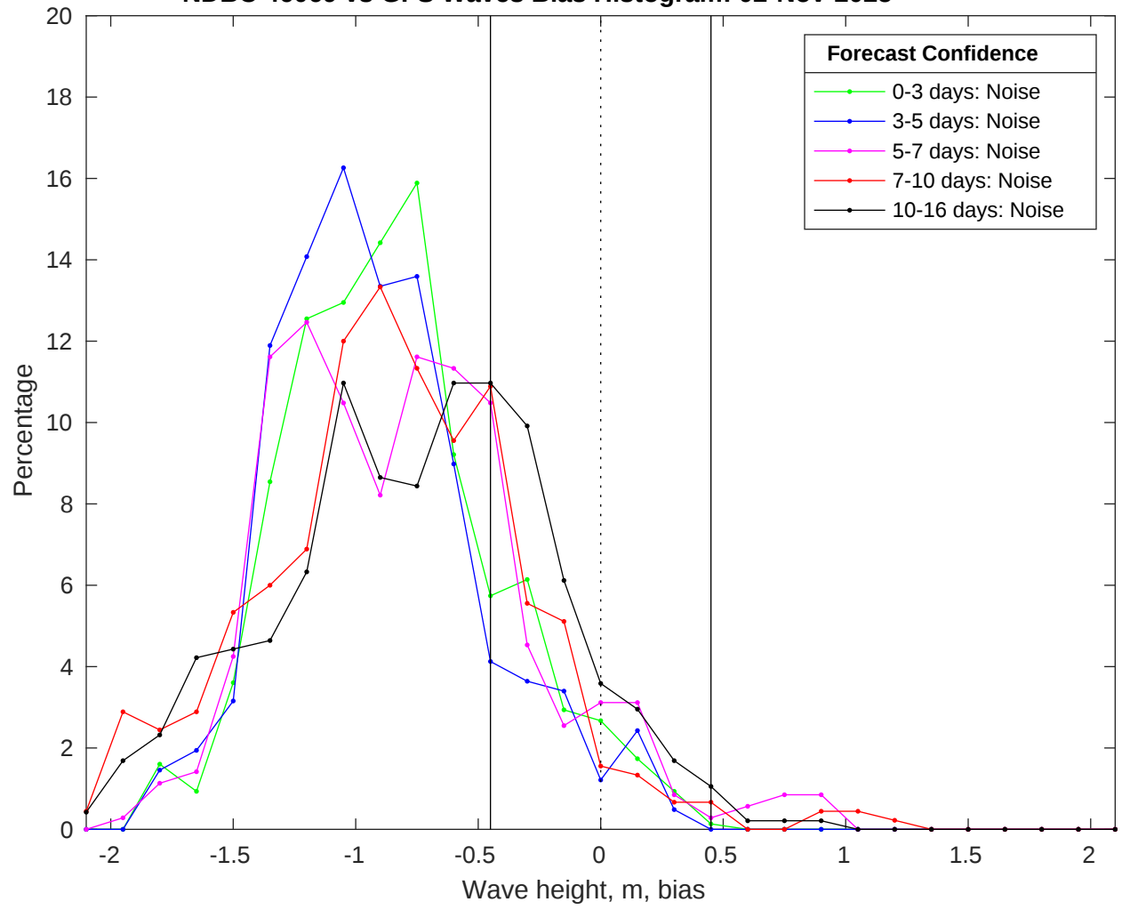
NDBC 46069 vs GFS Waves Bias Histogram: 02-Nov-2025
