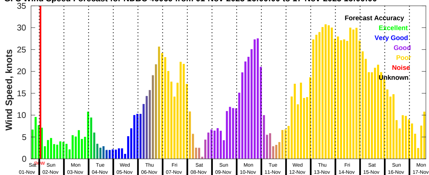
GFS Wind Speed Forecast for NDBC 46069 from 01-Nov-2025 16:00:00 to 17-Nov-2025 16:00:00
